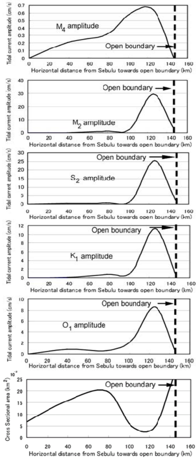
Fig.3 Spatial variation of M 4 , M 2 , S 2 , K 1 , and O 1 tidal current amplitudes and cross-sectional area along the axis of the Mahakam estuary.
